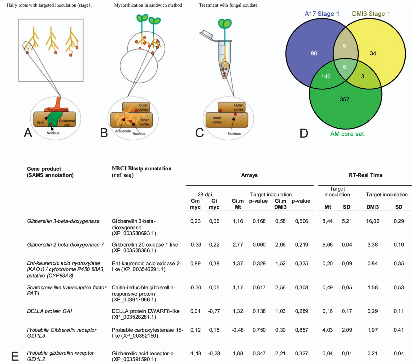
Figure 1. The drawings (A-C) illustrate the setup developed to detect gene expression, while D-E summarize the main expression results. (A) M. truncatula hairy roots inoculated with Gi. margarita spores at specific root sites. The fungus develops a hyphopodium and the epidermal cell reacts by producing the PPA. (B) The sandwich method leads to a full colonization in 28d, allowing the formation of branched arbuscules inside cortical cells. (C) M. truncatula seedlings treated with fungal exudates produced by germinating spores. (D) Venn diagram summarizing the transcriptional responses of M. truncatula roots sampled at stage 1, showing the numbers of genes activated in different conditions: M. truncatula WT versus Mtdmi3 mutant roots at fungal contact stage and versus the whole AM core set identified by Hogekamp et al. (2011) in fully mycorrhizal roots. (E) The table lists the genes detected in the two array experiments and validated with RT-Real time. (i) Medicago truncatula at 28dpi with G. mosseae (Gm myc) and G. intraradices (Gi myc) (Hogekamp et al., 2011); and (ii) targeted inoculation of M. truncatula transformed roots with Gi. margarita (Gi.m) and sampled at hyphopodium contact, as well as of M. truncatula MtDmi3 mutant transformed roots (Gi.m DMI3).
